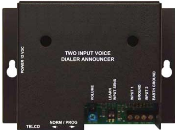
TAK-4202 Telephone Auto Dialer Unit
