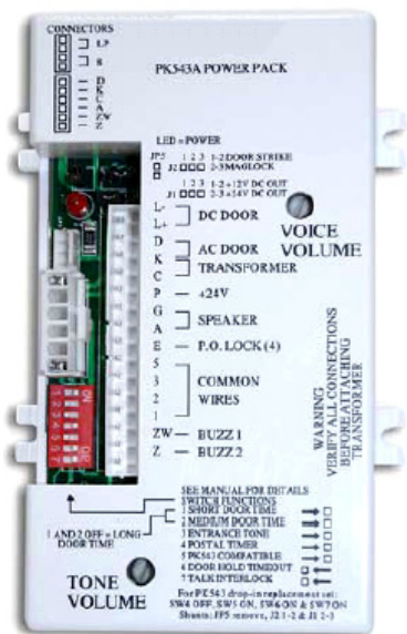
PK543A Intercom Amplifier (shown without wiring harness)
