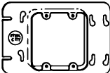
IH355 Plaster Ring
