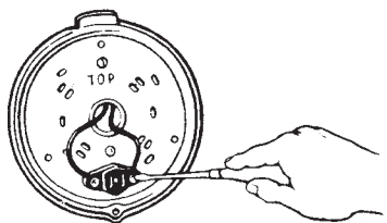
1. Pull wires through spacious center hole and connect to large binding posts.
